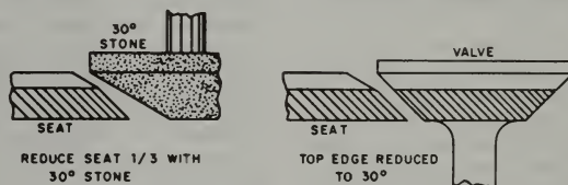
FIGURE 10-11. Grinding top surface of the valve seat.
